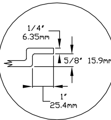
Close-up view of nailing flanges on acrylic models
